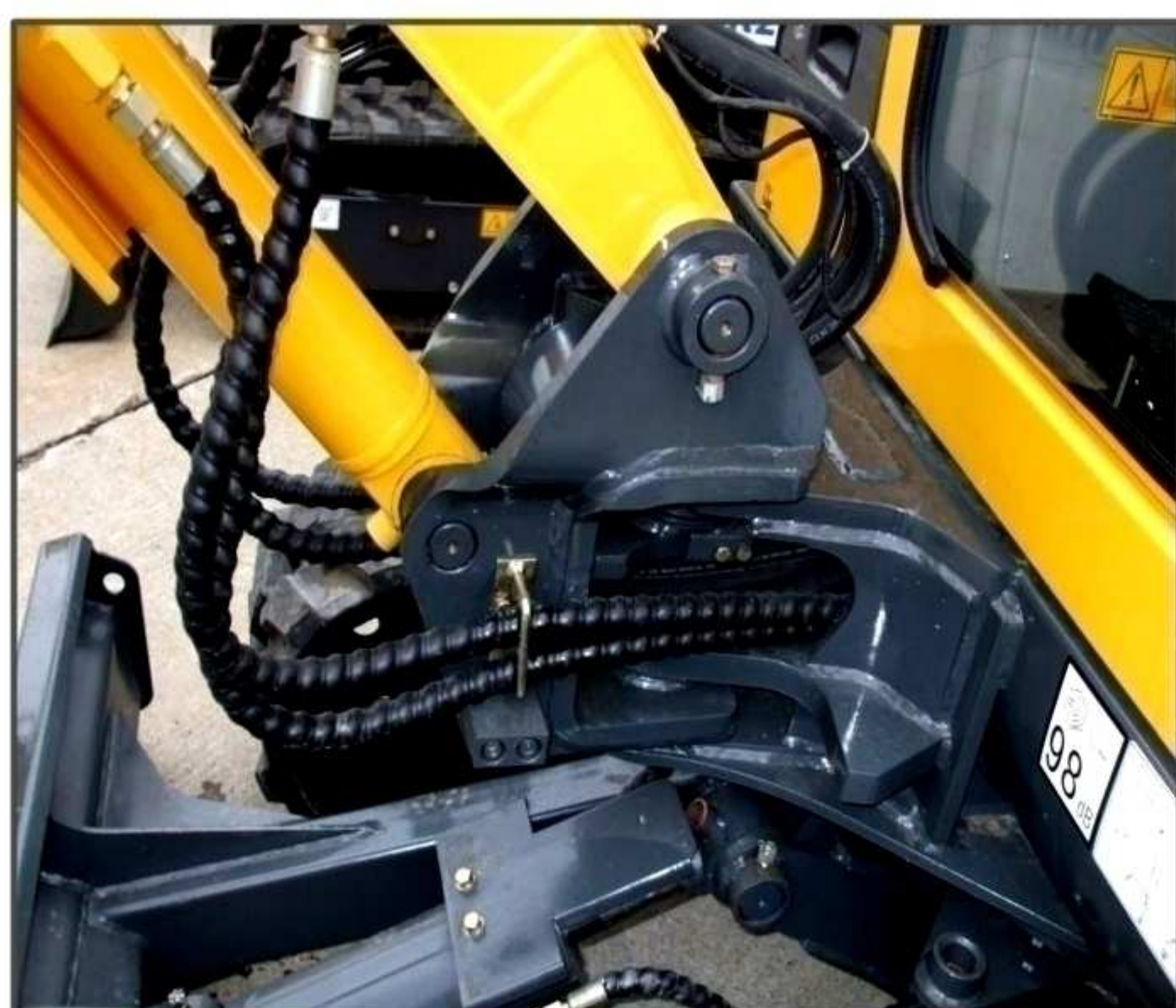
Hydromatic-Hydraulik
